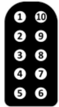
VIEW FROM REAR OF CONNECTOR
