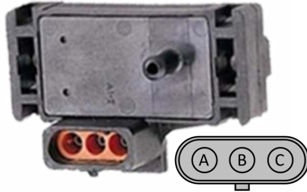
GM MAP Sensor Tower Plug
