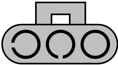
CONNECTOR INDEXING SLOT DETAIL. VIEW OF FRONT.
